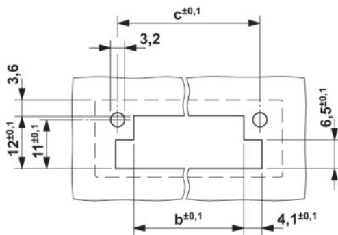
Drilling plan/solder pad geometry
