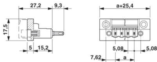
Dimensioned drawing
